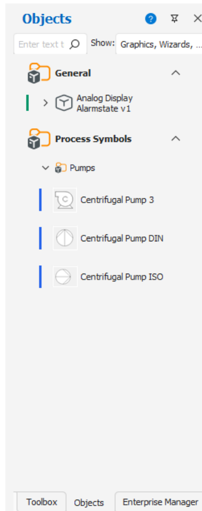
Figure 1: Objects Toolbox
